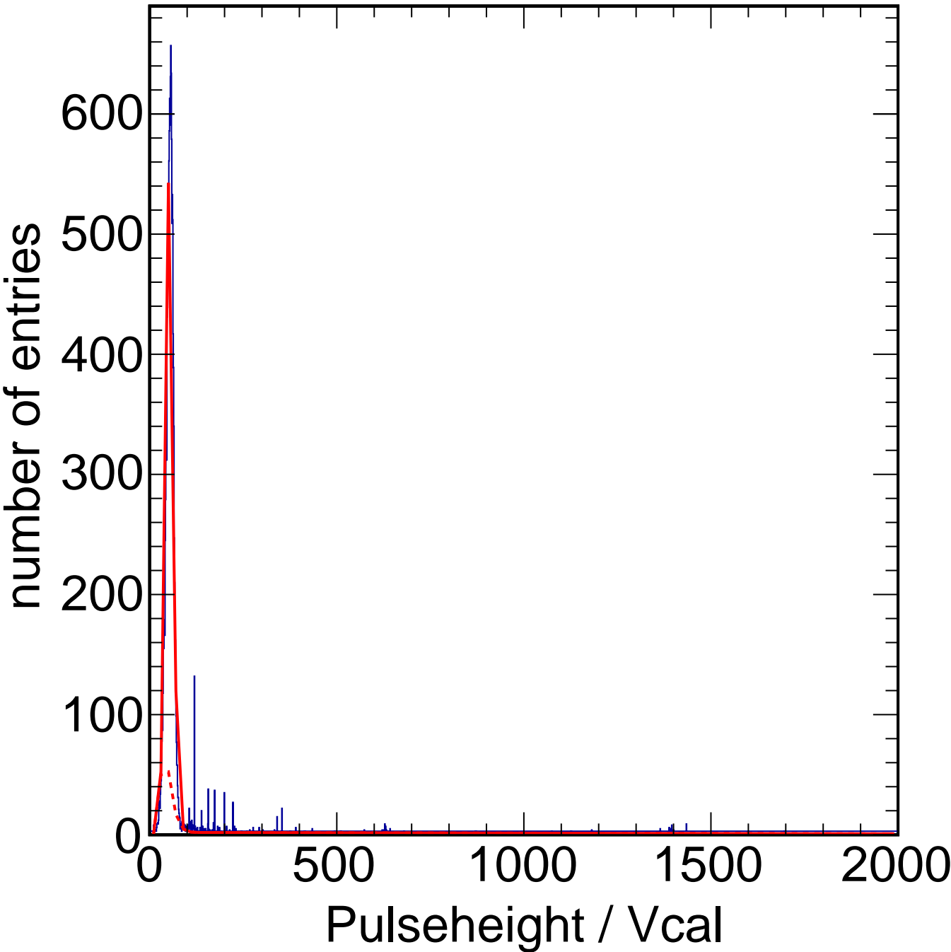
X-ray Calibration - Target Zn Method Spectrum Chip C2
