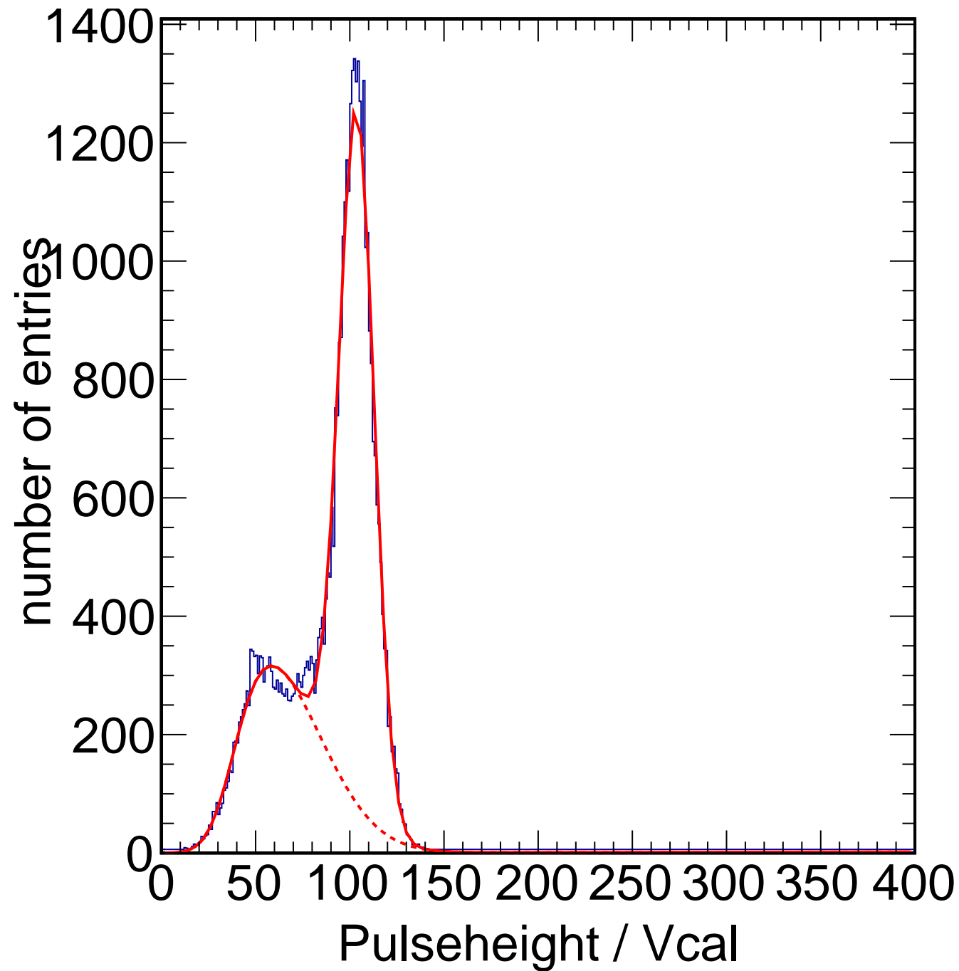
X-ray Calibration - Target Mo Method Spectrum Chip C10
