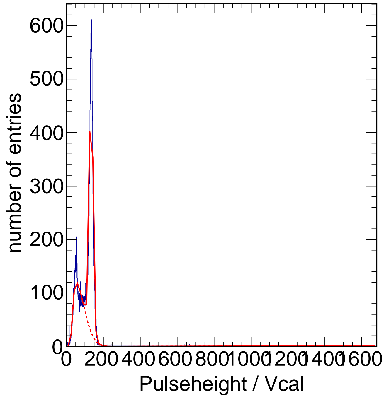
X-ray Calibration - Target Ag Method Spectrum Chip C8
