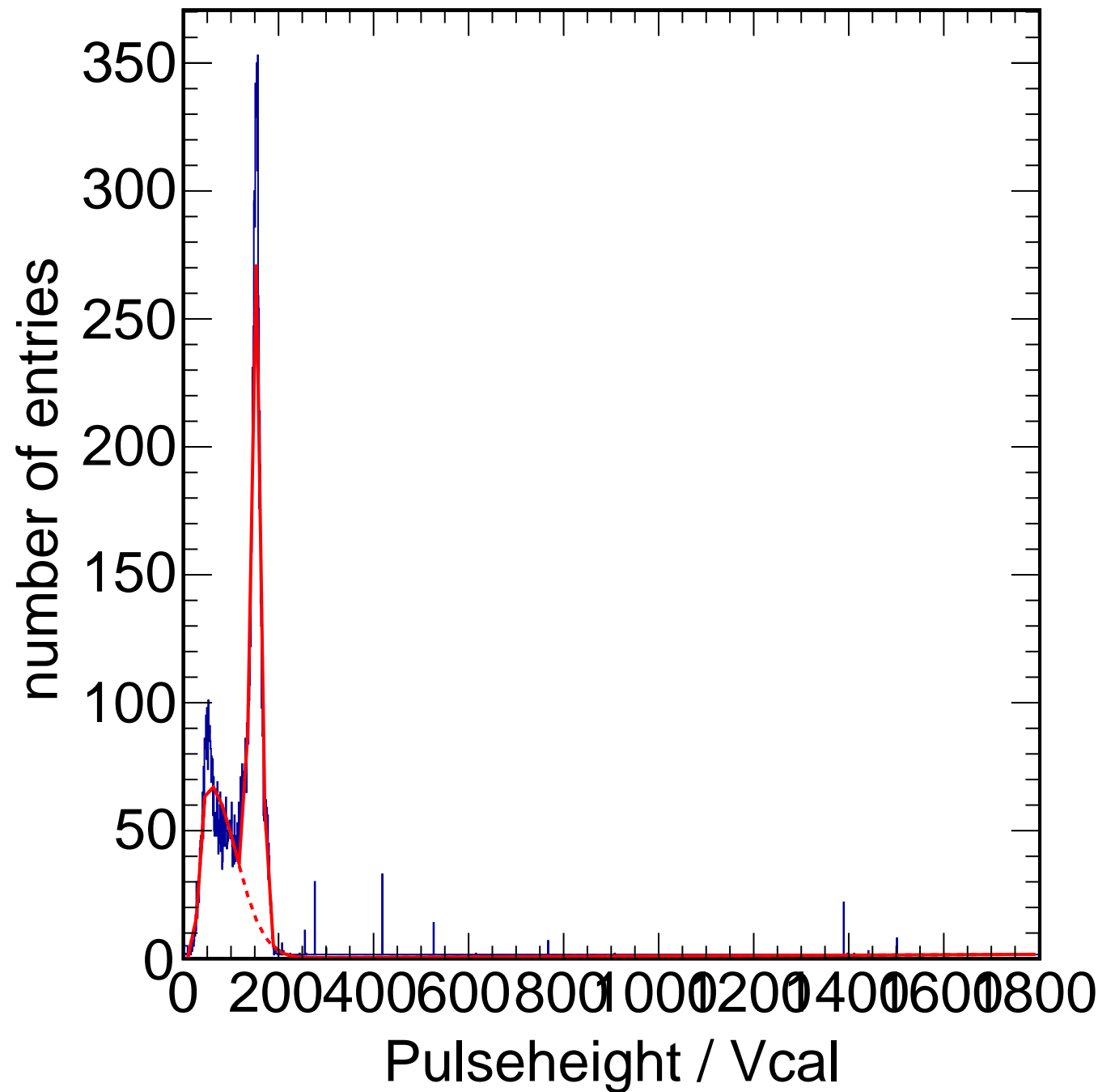
X-ray Calibration - Target Sn Method Spectrum Chip C6
