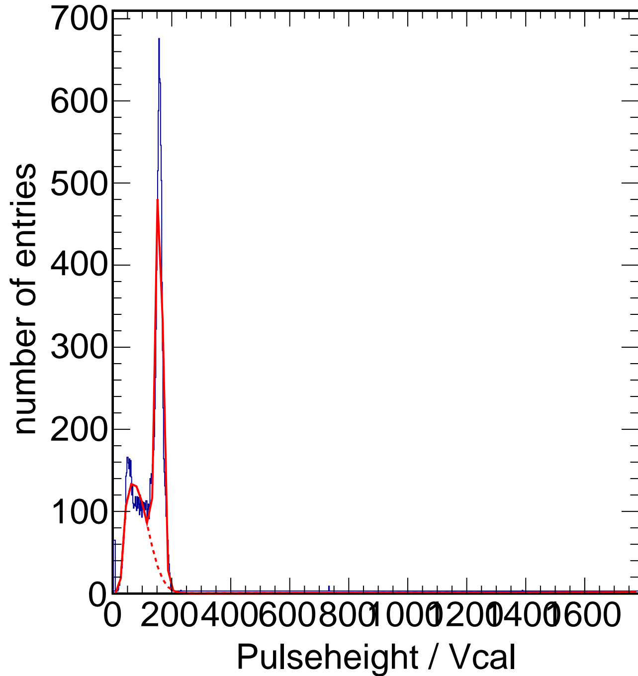
X-ray Calibration - Target Sn Method Spectrum Chip C5
