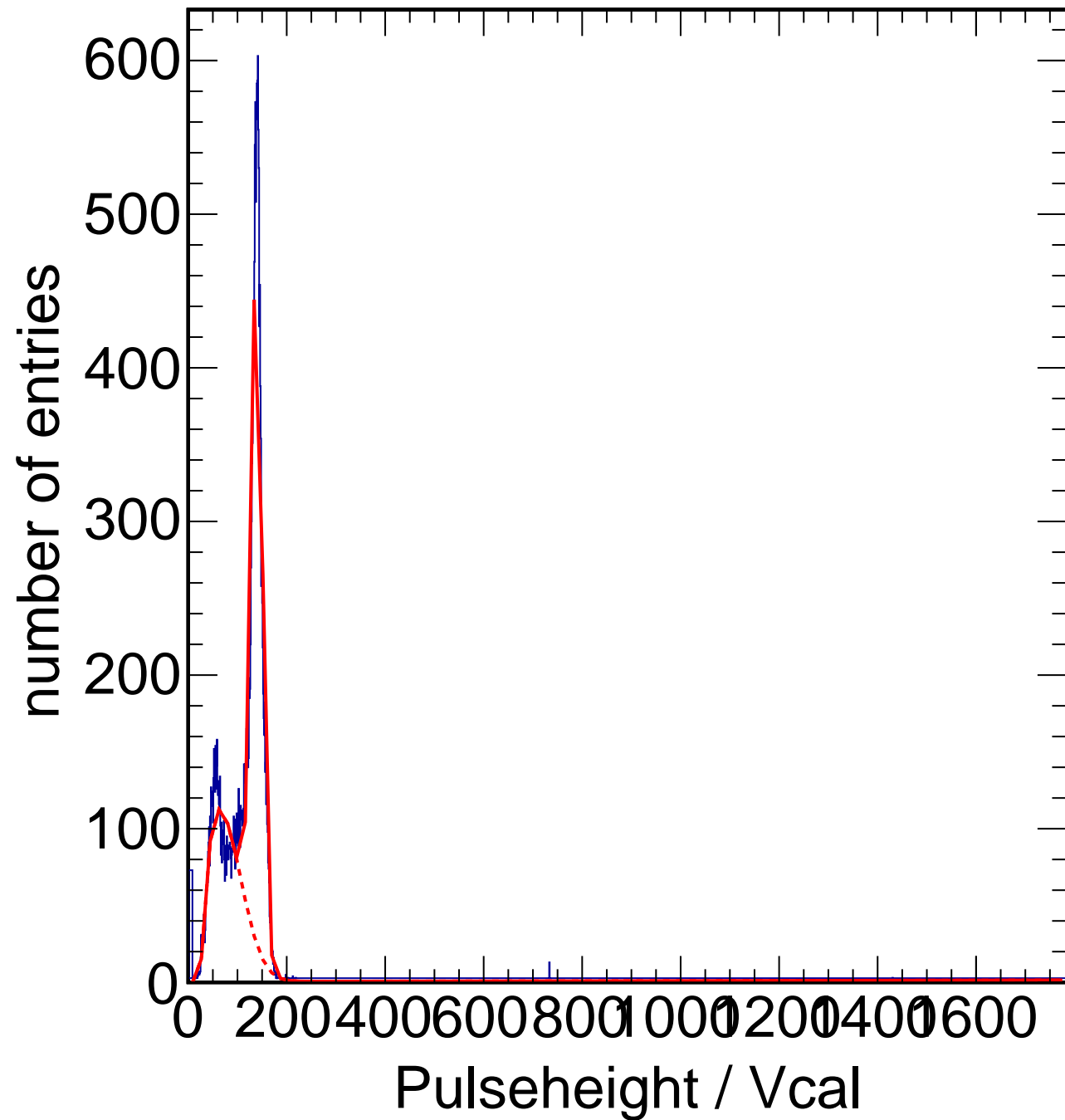
X-ray Calibration - Target Ag Method Spectrum Chip C5
