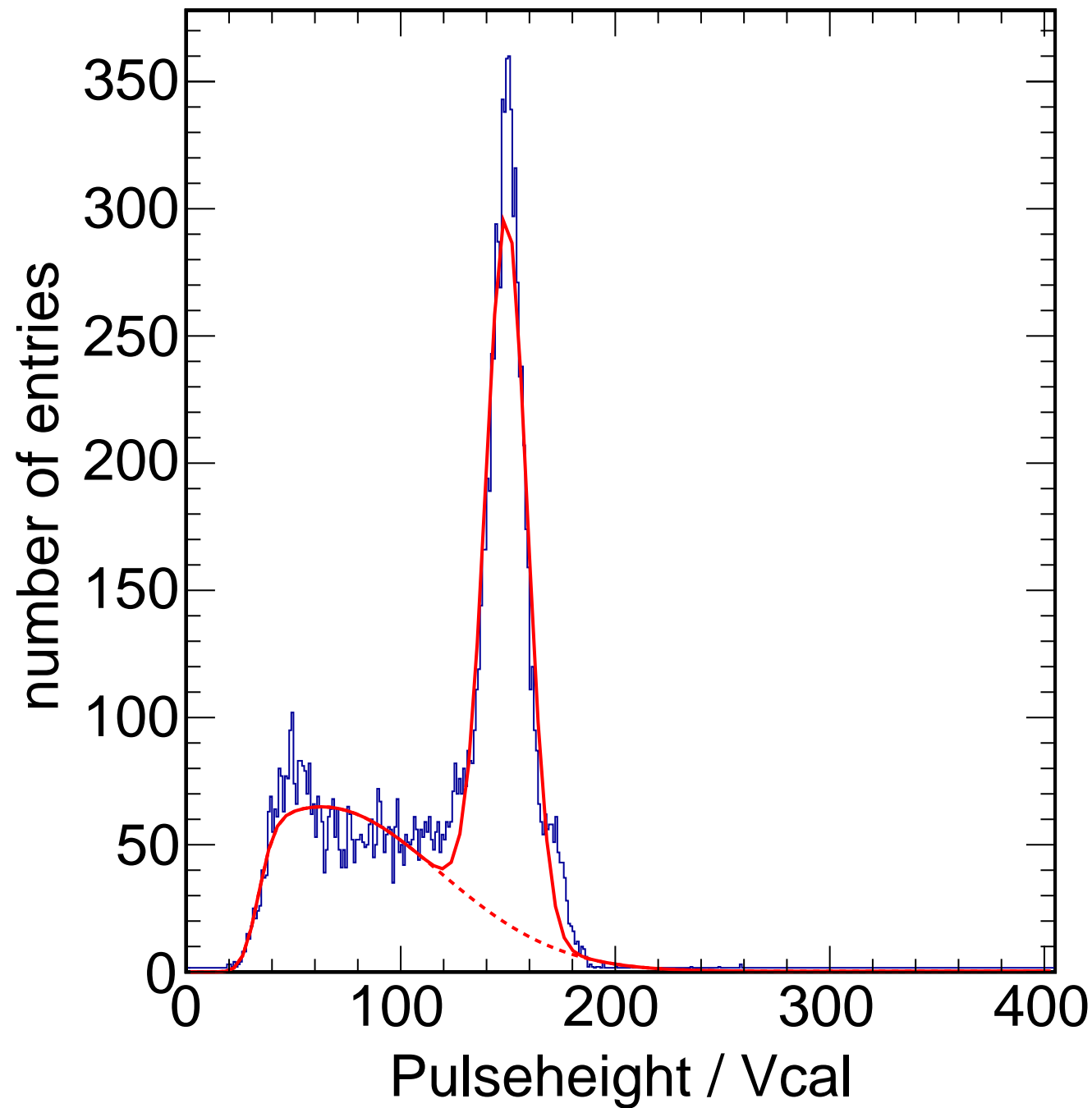
X-ray Calibration - Target Sn Method Spectrum Chip C4
