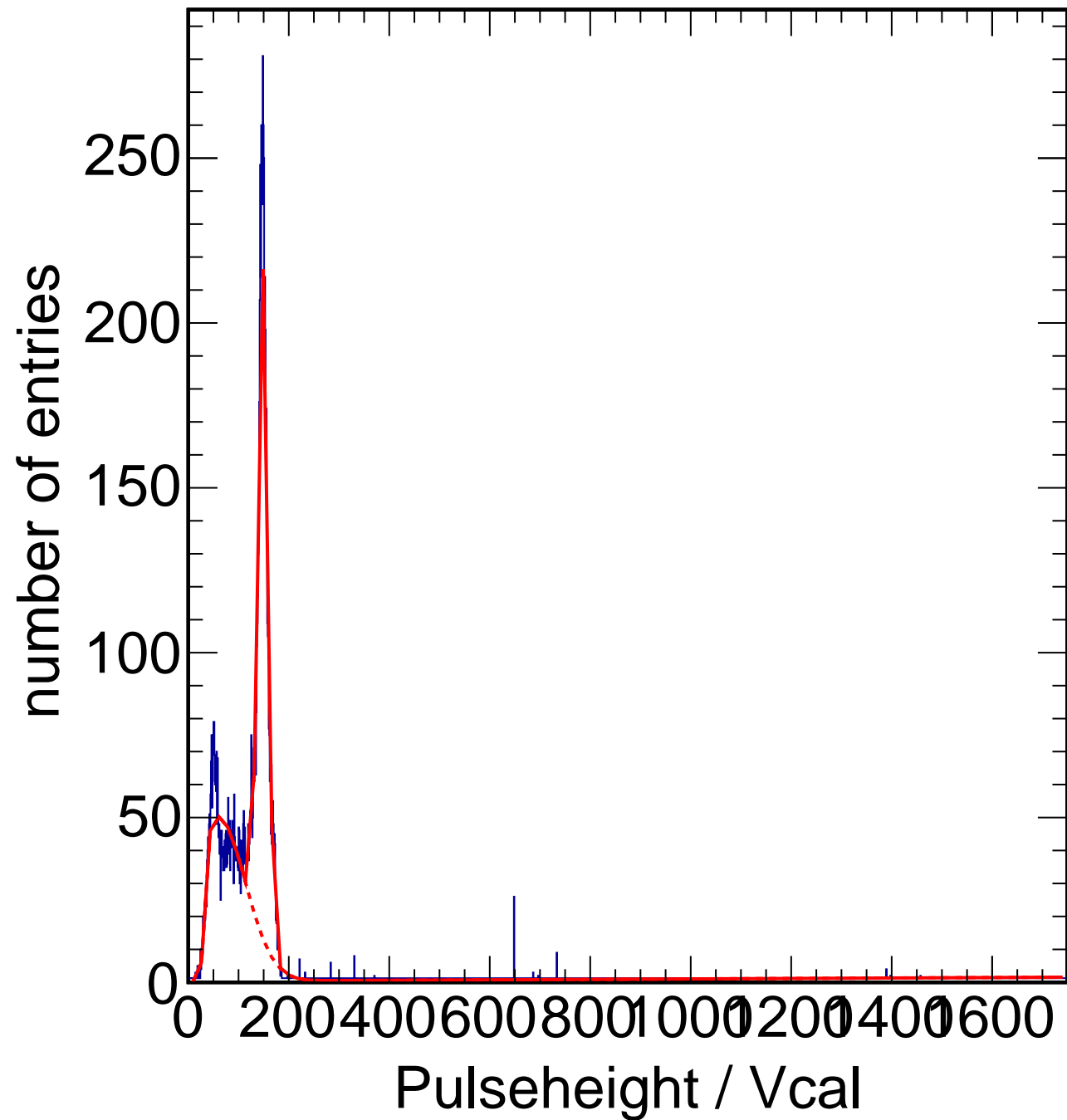
X-ray Calibration - Target Sn Method Spectrum Chip C13
