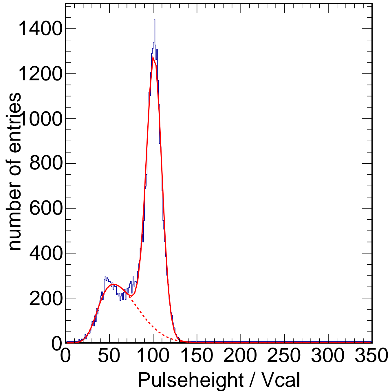
X-ray Calibration - Target Mo Method Spectrum Chip C12
