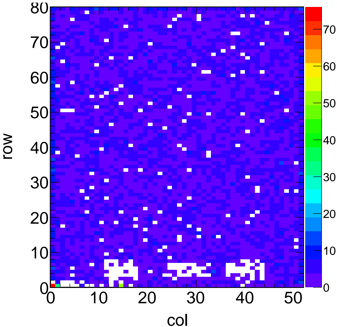
X-ray Hit Map - Target Sn Method Spectrum Chip C10
