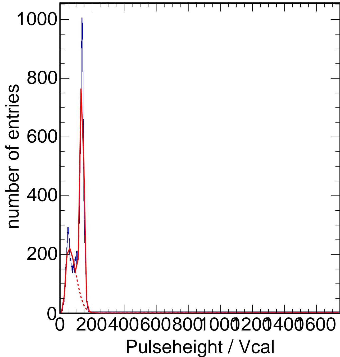
X-ray Calibration - Target Ag Method Spectrum Chip C9
