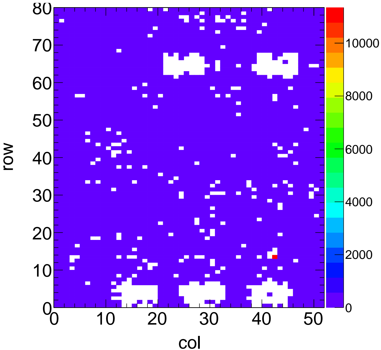
X-ray Hit Map - Target Zn Method Spectrum Chip C6
