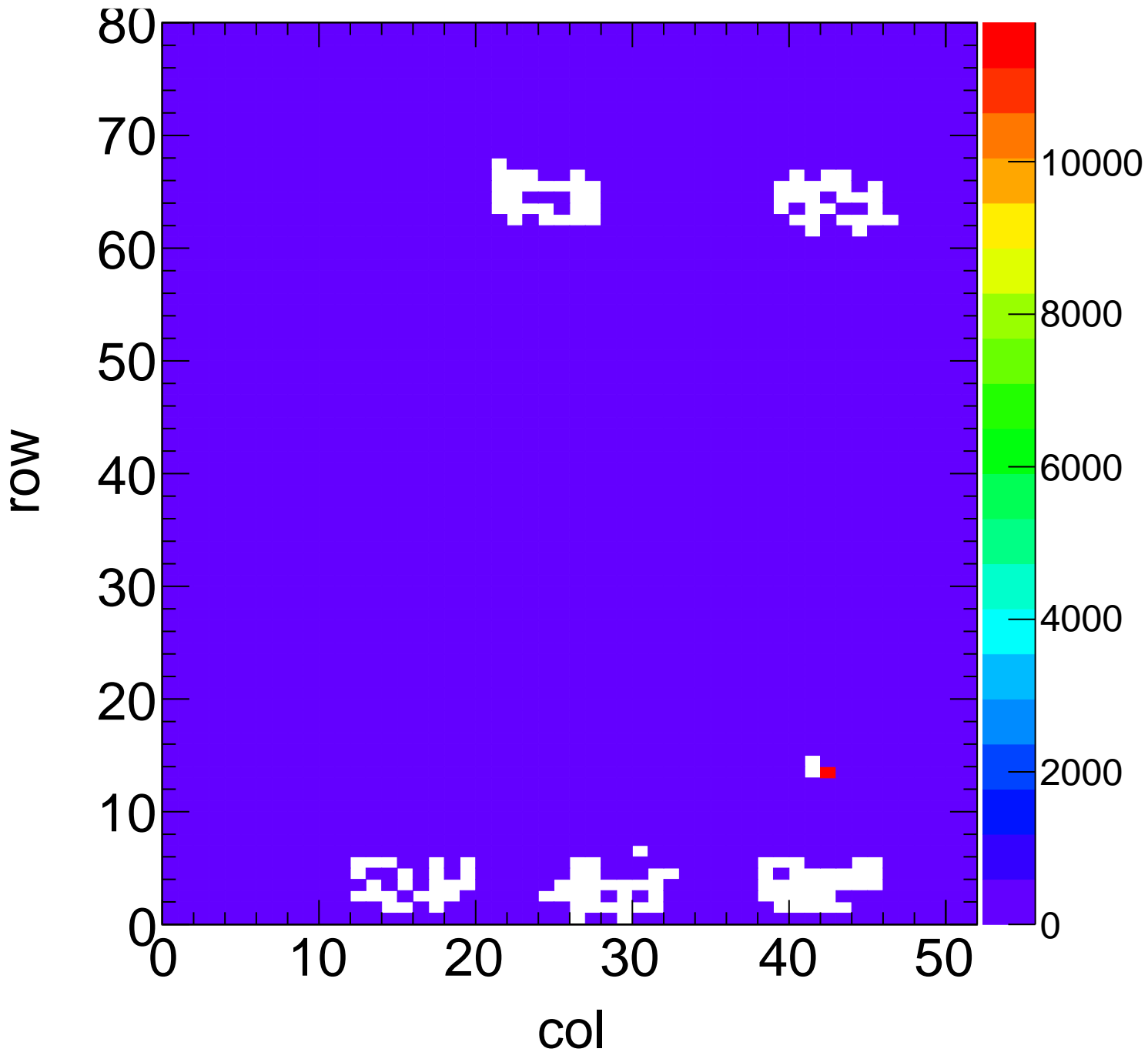
X-ray Hit Map - Target Mo Method Spectrum Chip C6
