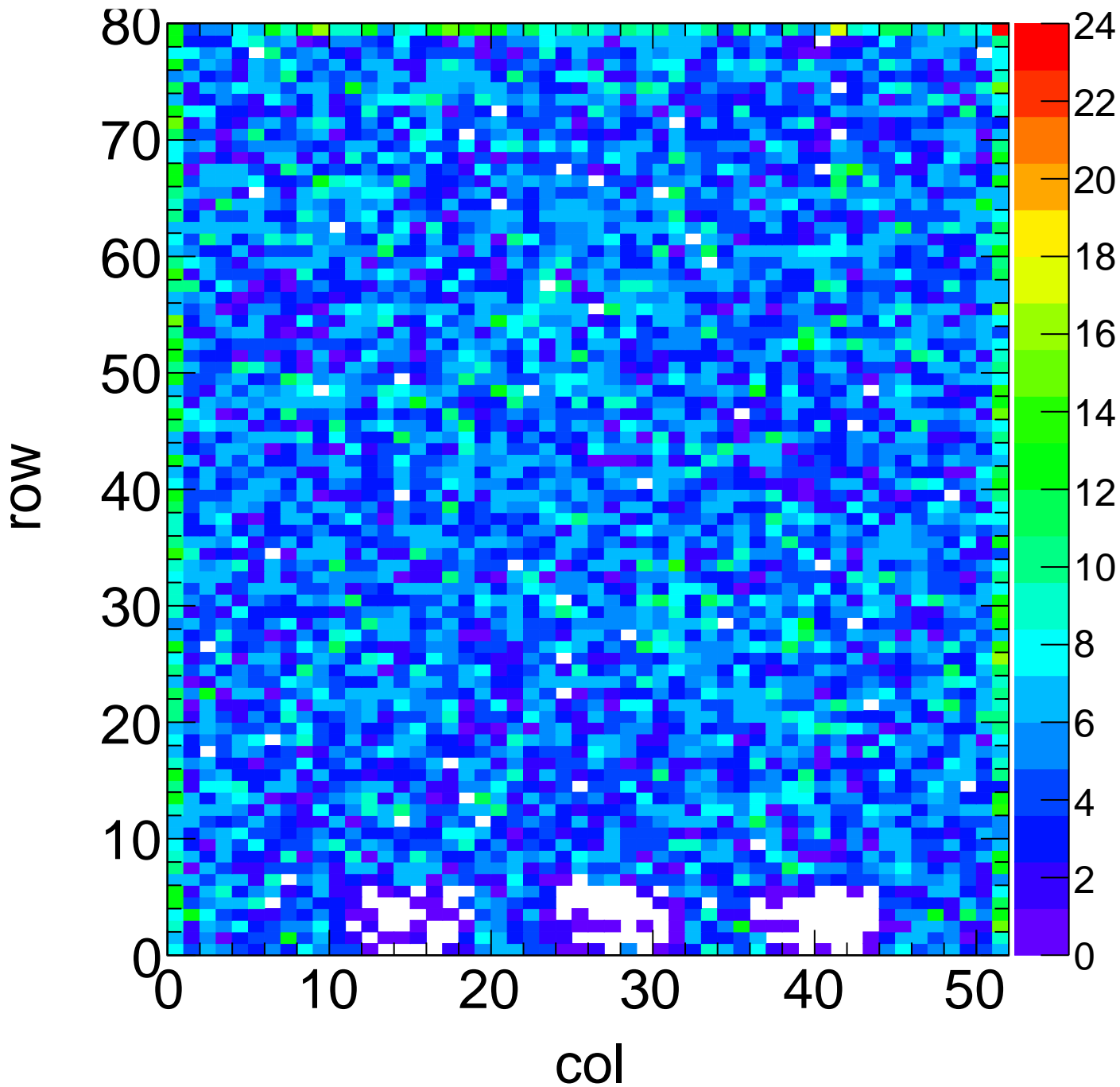
X-ray Hit Map - Target Ag Method Spectrum Chip C5
