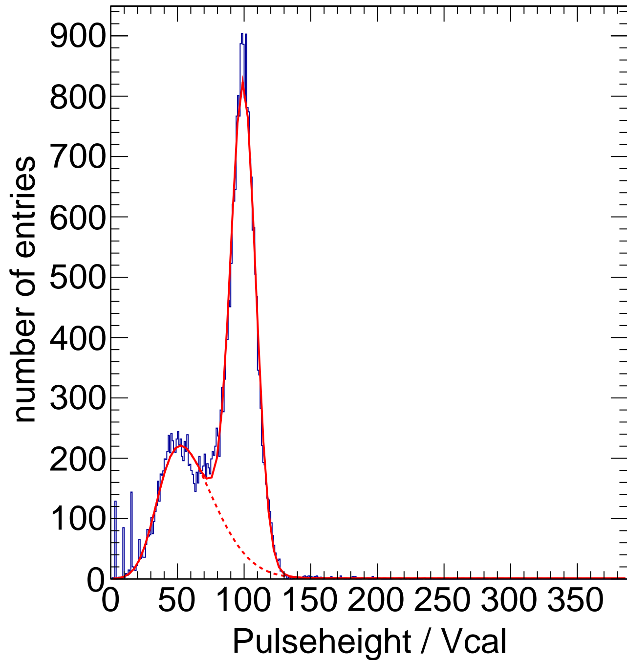
X-ray Calibration - Target Mo Method Spectrum Chip C14
