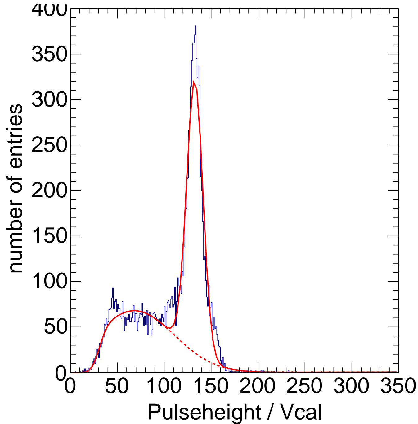
X-ray Calibration - Target Sn Method Spectrum Chip C9
